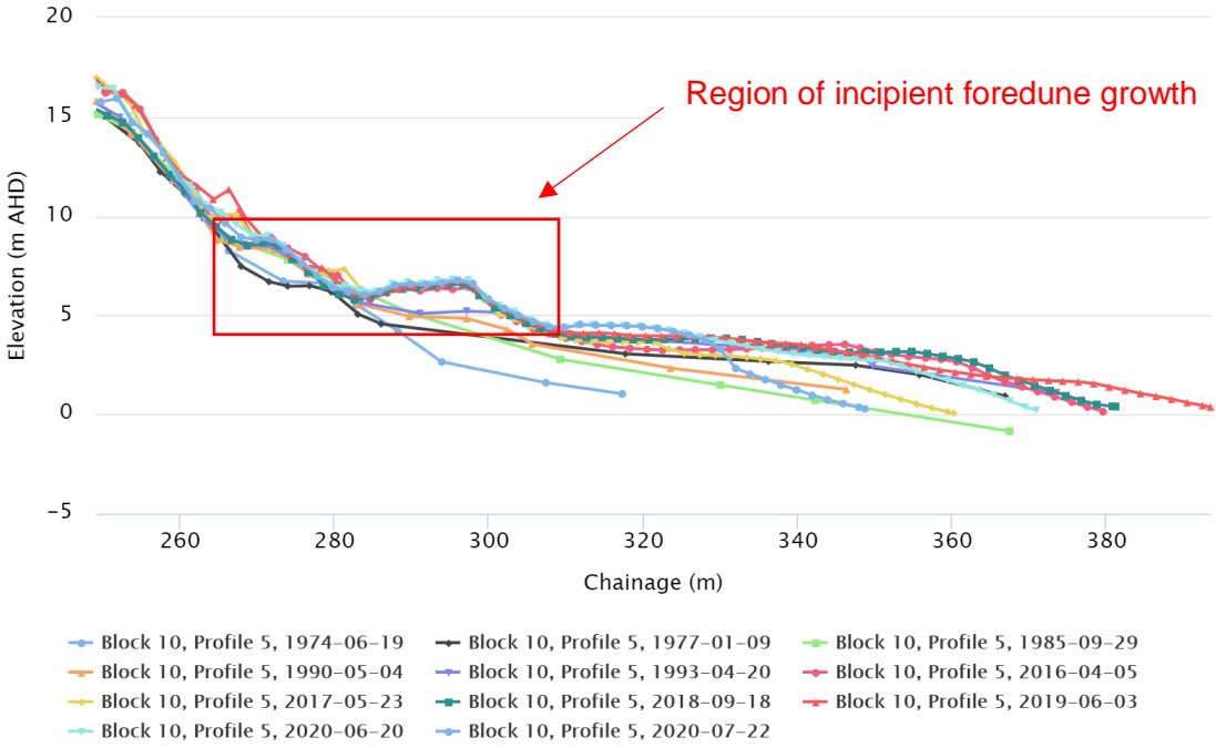
Figure 3.4: Foredune growth at Profile 10-5 north of Wamberal Lagoon.
