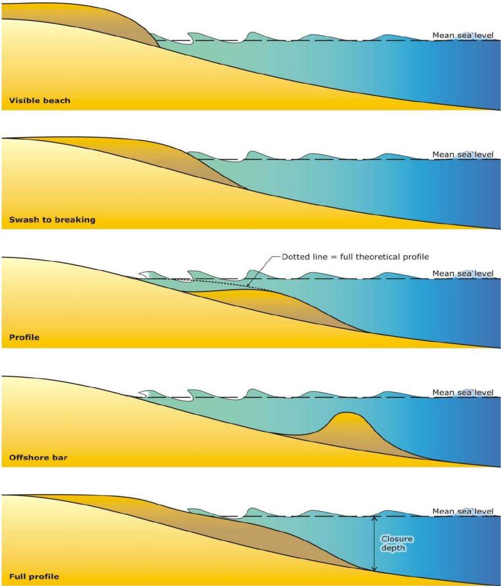
Figure 2.2: Alternative beach fill placement locations. From Carley and Cox (2017).
